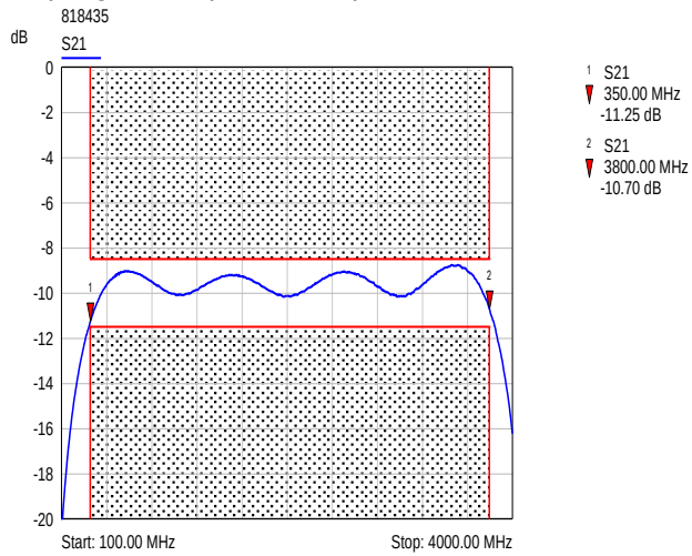
Coupling 10 dB (BN818435): S21
