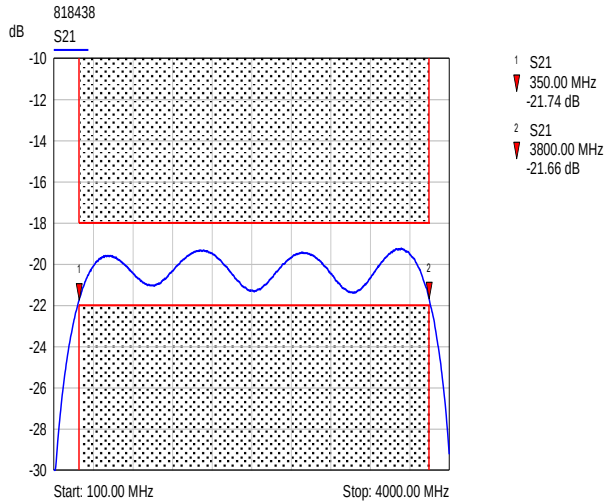
Coupling 20 dB (BN818438): S21
