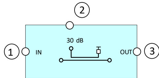
Block diagram using 30 dB as example
